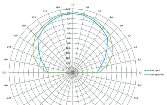
ANTENNA RADIATION PATTERN
